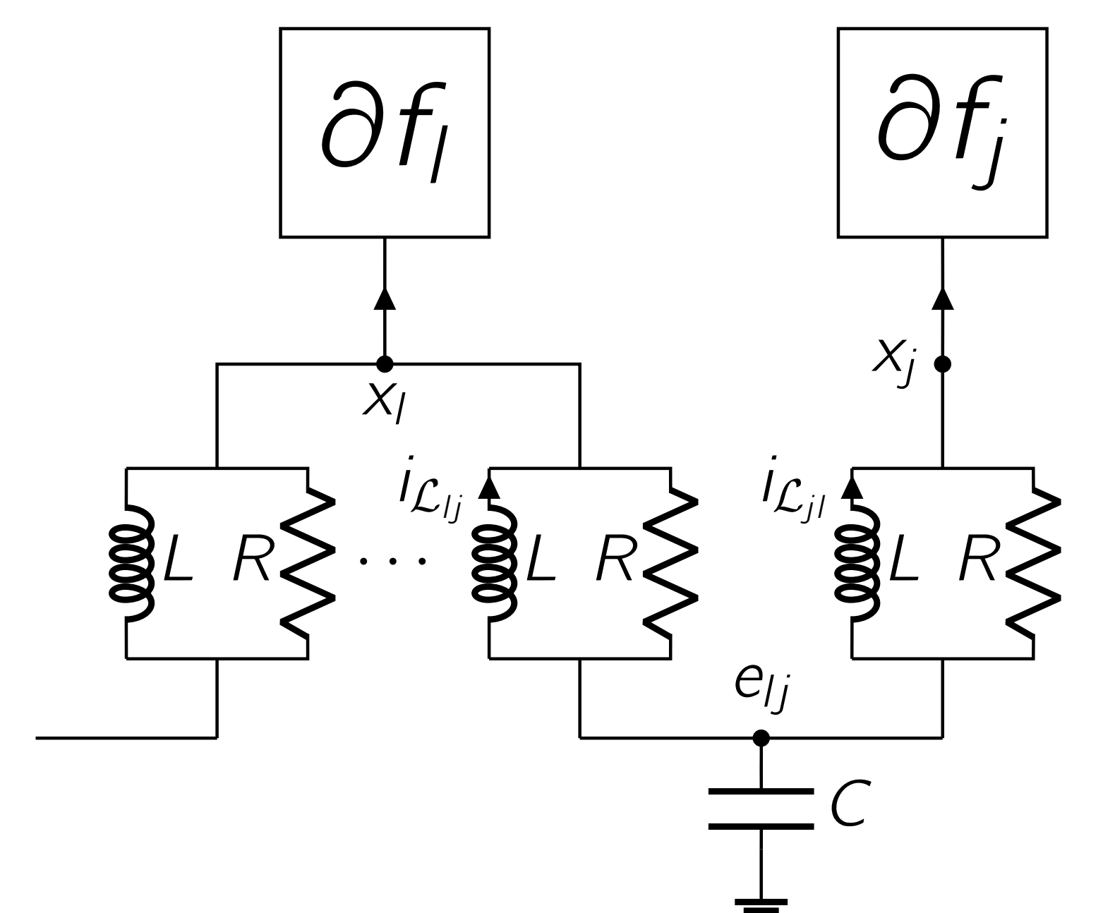
DADMM+C (new!)
