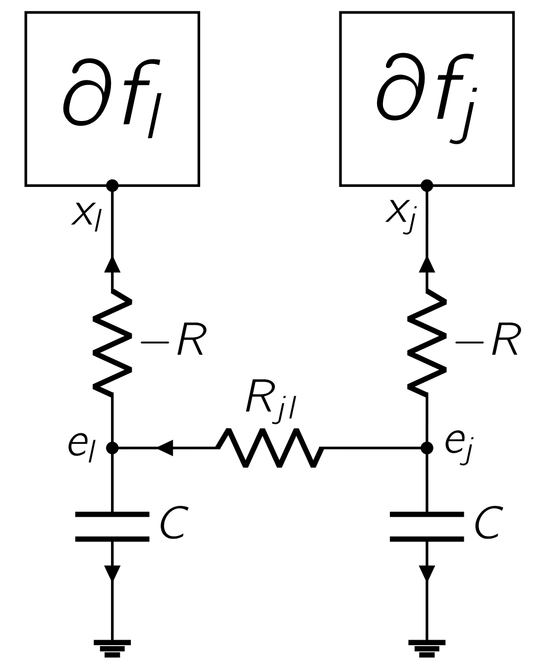
Decentralized ADMM
