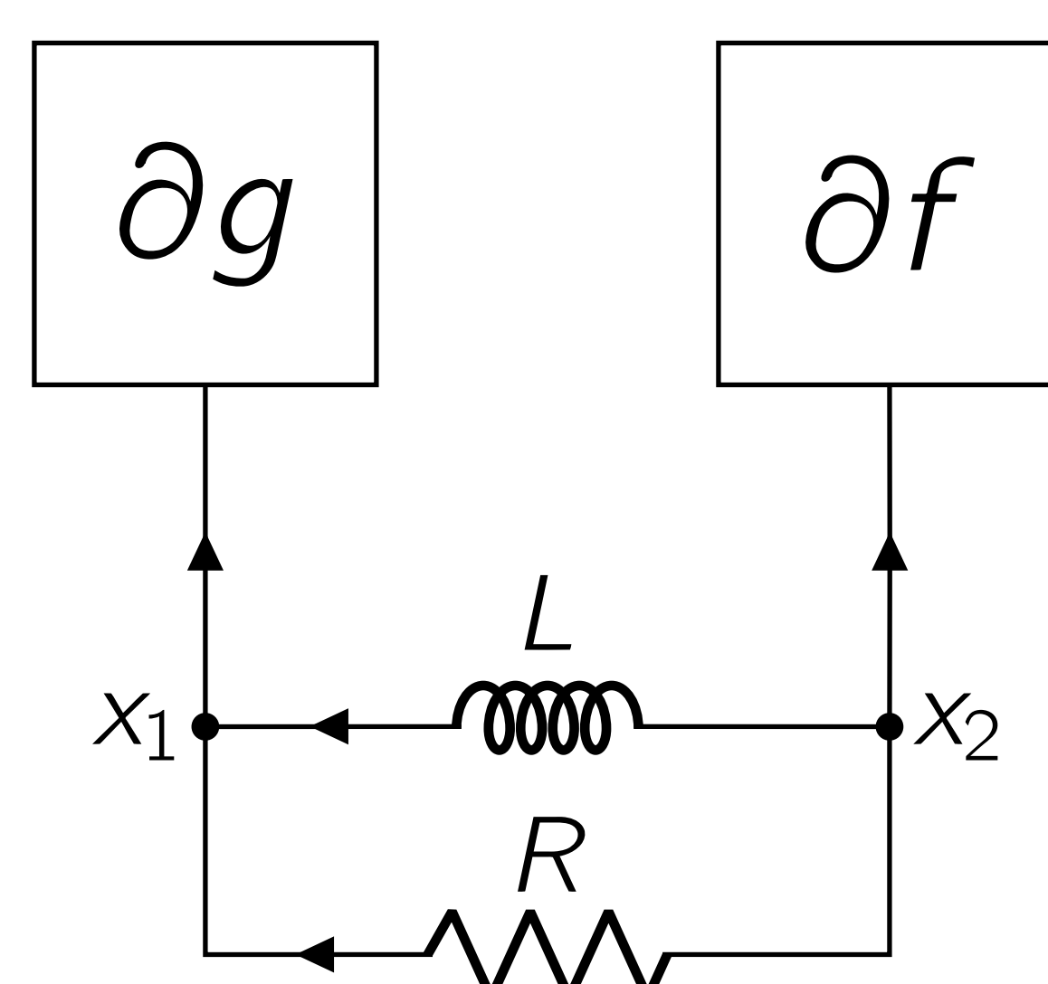
Davis-Yin splitting
