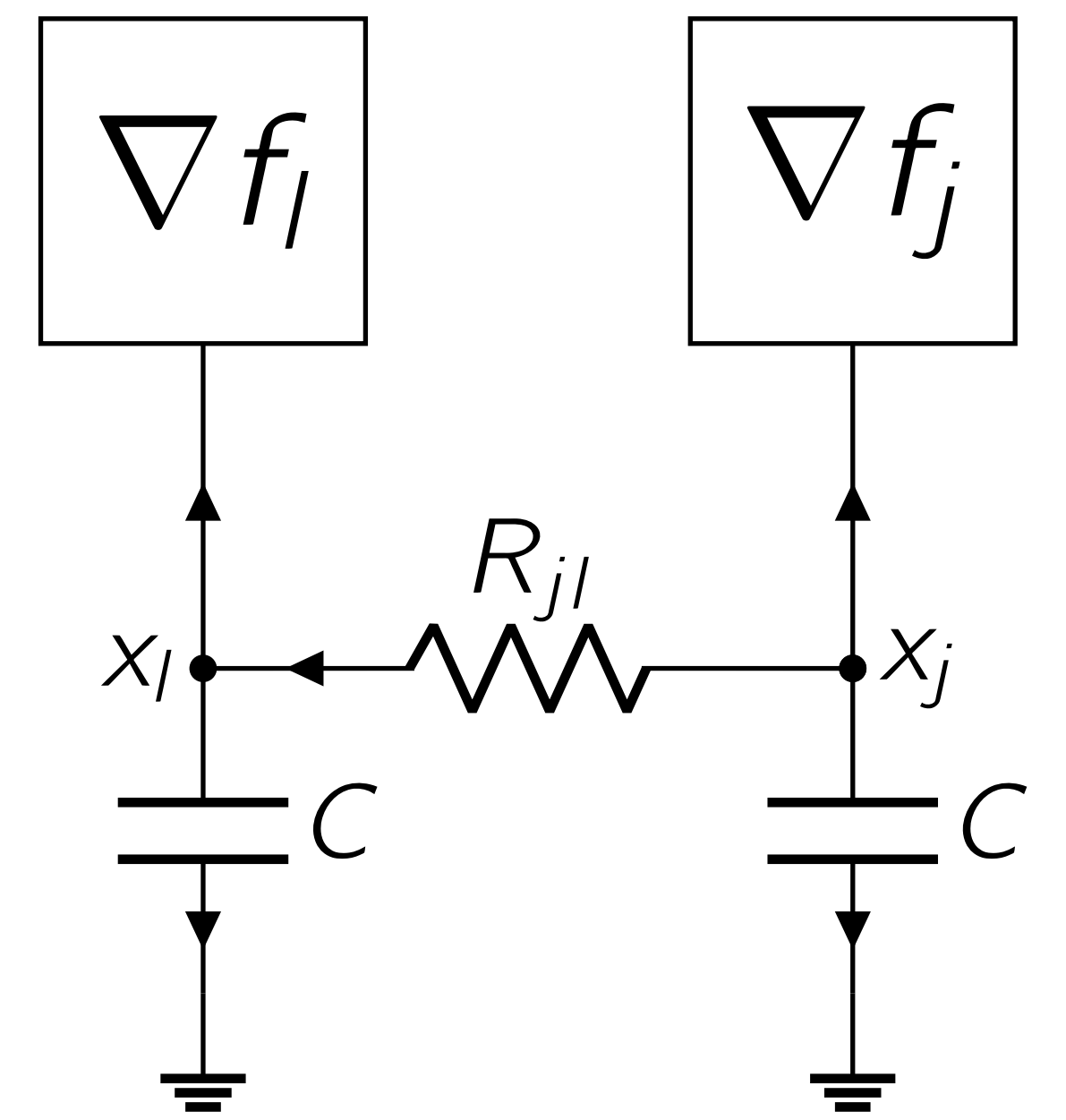
Adapt-then-combine
