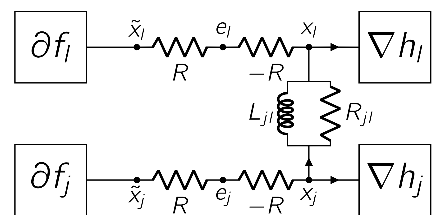
PG-EXTRA
