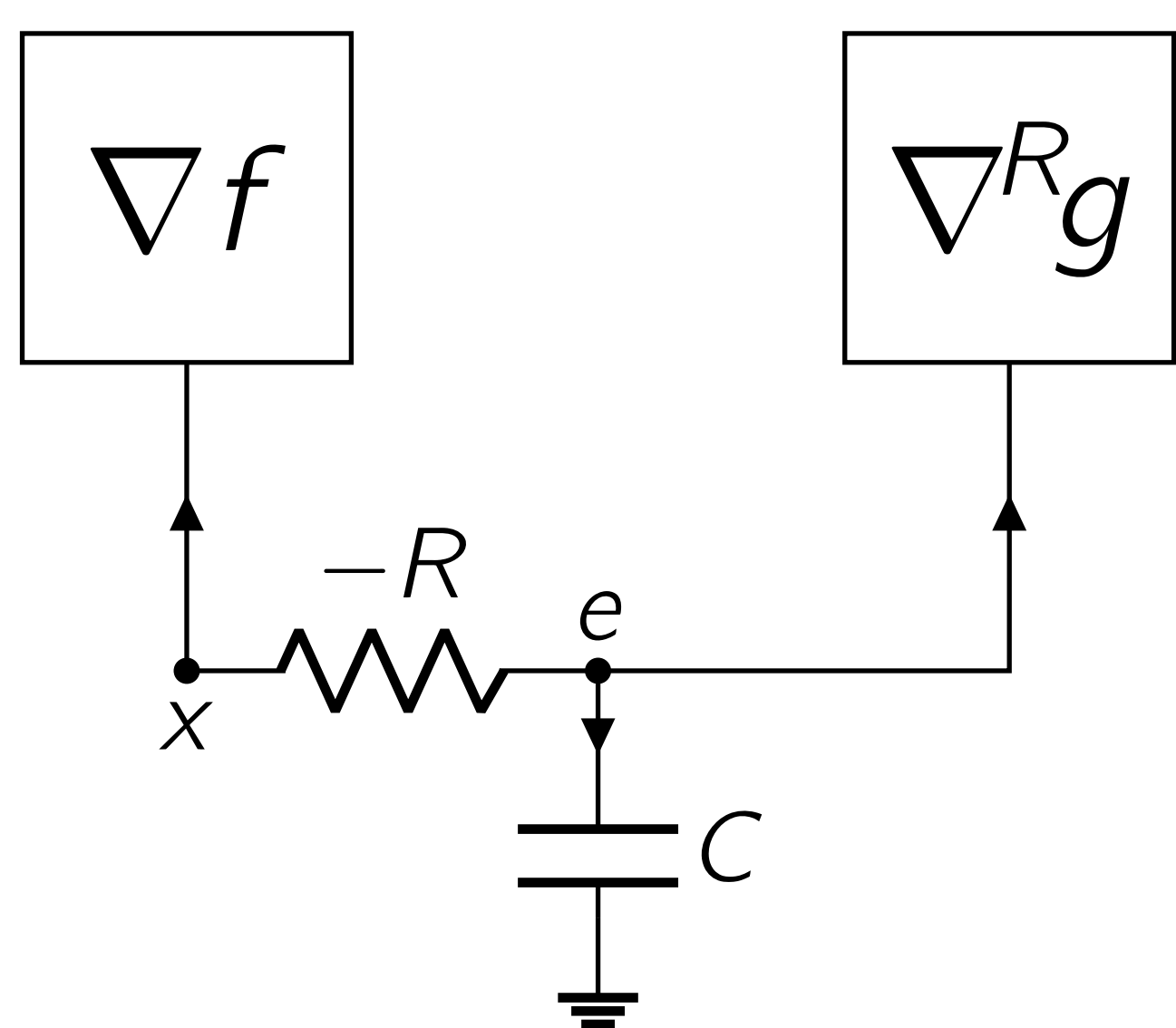
Your algorithm
