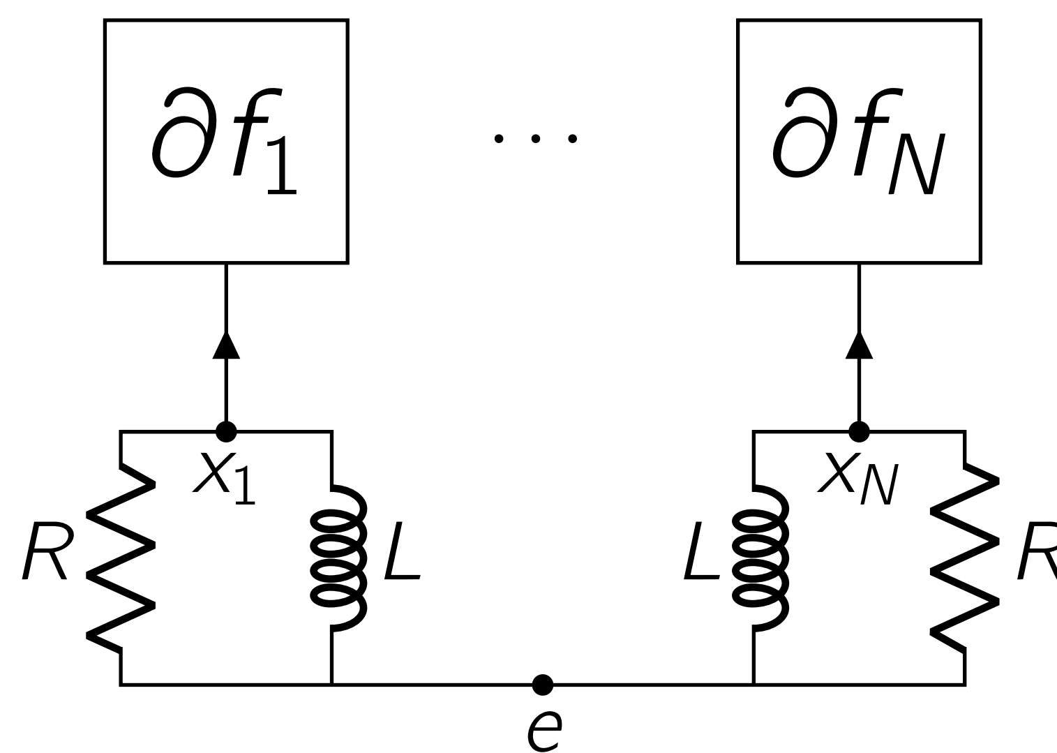
Douglas-Rachford splitting
