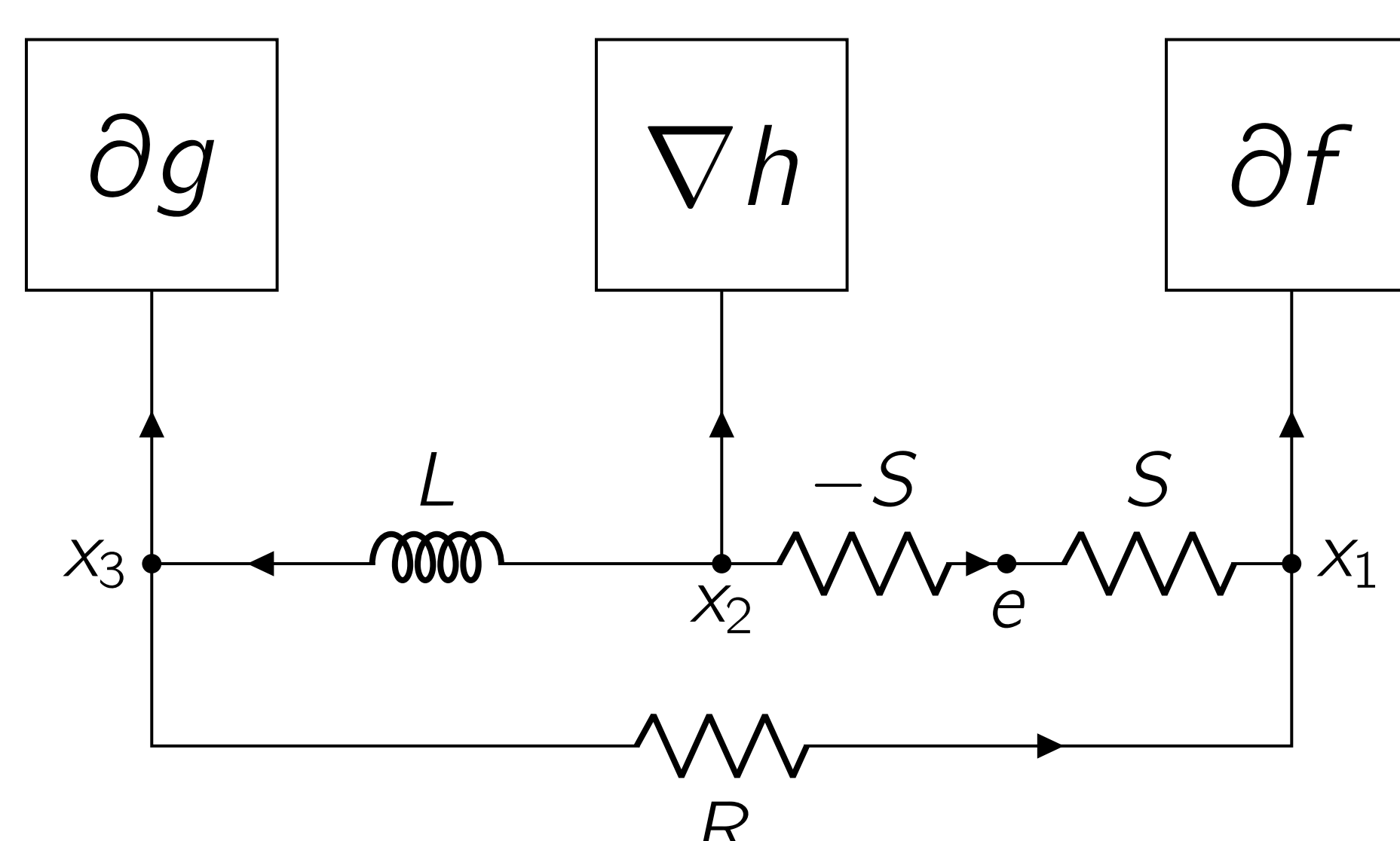
Davis-Yin splitting
