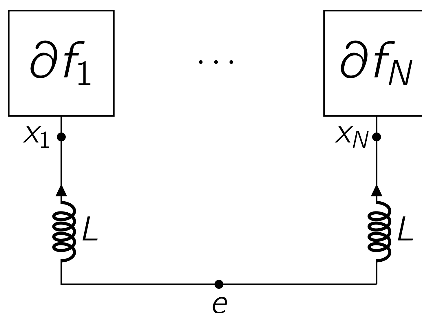
Prox Decomposition
