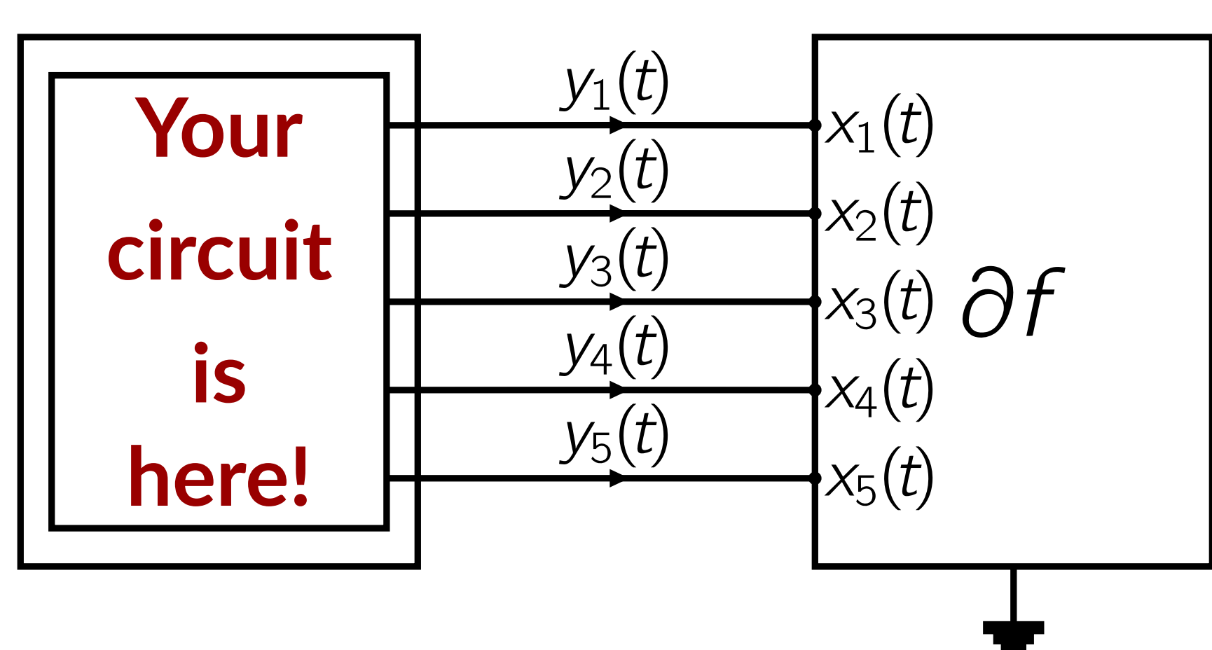
Your algorithm
