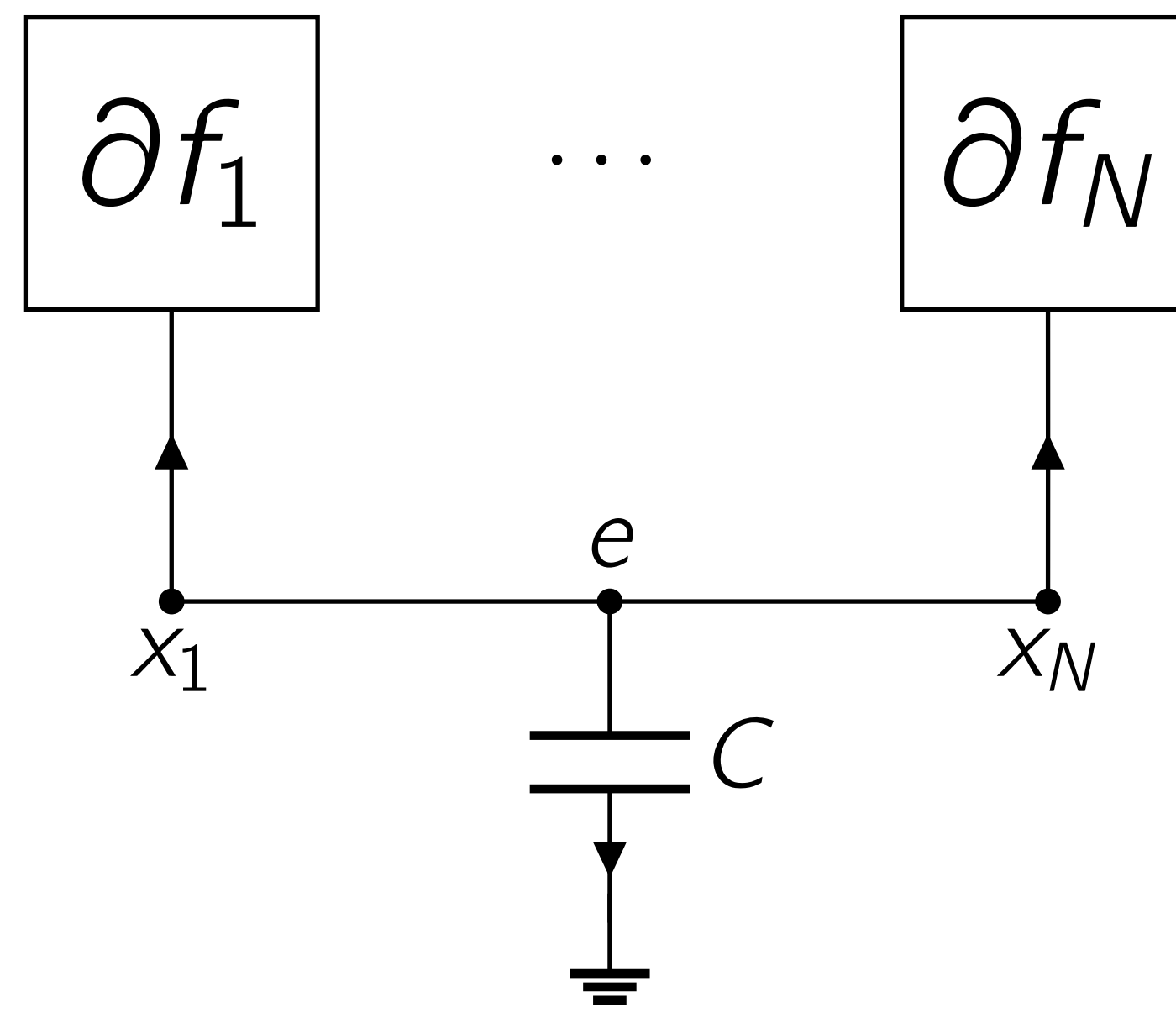
Dual Decomposition
