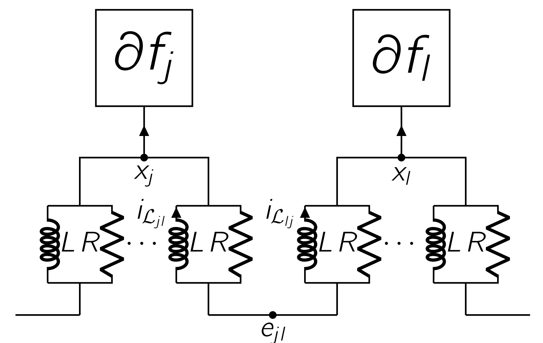
PG-EXTRA
